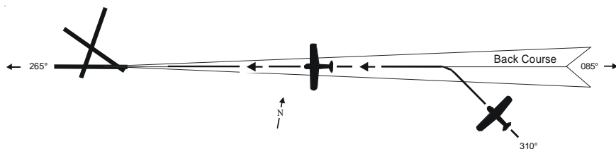
Fig. 3-17. AP Display, REV APR Mode Engaged, Track LOC Back Course Inbound
