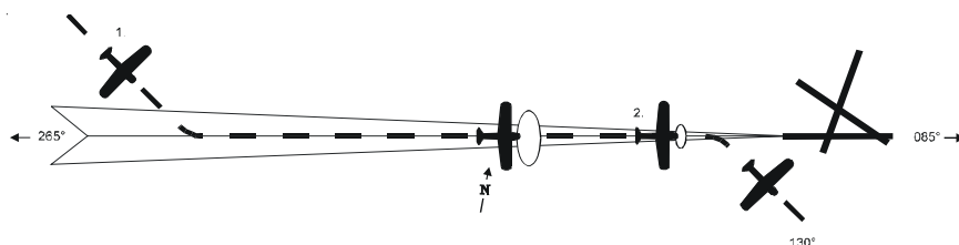
Fig. 3-26. AP Display, NAV APR Mode Engaged, Track LOC Front Course Inbound
