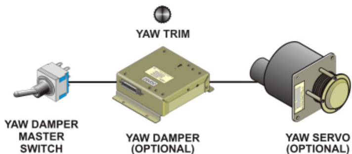
Fig. 1-2. Yaw Damper Block Diagram
